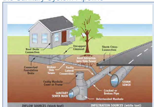
Figure 4. Inflow and Infiltration Sources to the Sanitary System Pipeline
