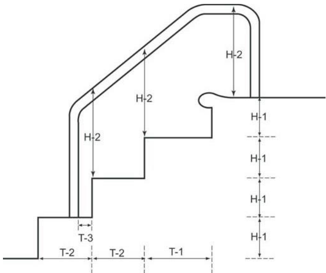
FIGURE 31-7 STAIR AND HANDRAIL DIMENSIONS
