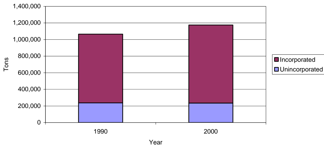
CO 2 Emissions from Energy Use
