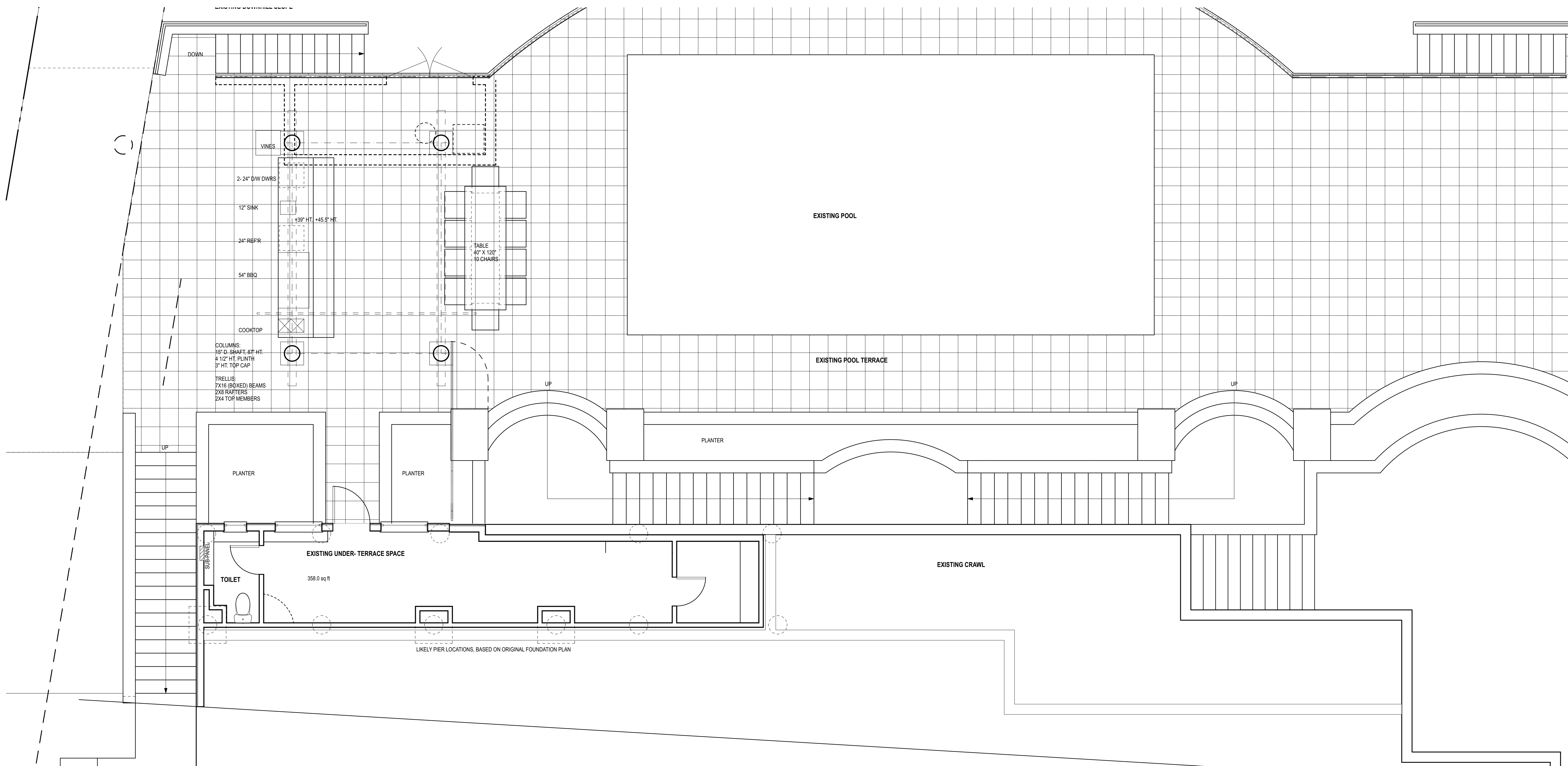
1 A1.1 EXISTING POOL TERRACE PLAN SCALE: 1/4" = 1'-0"
