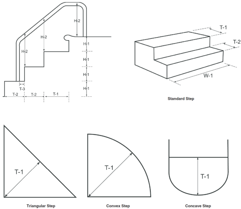
Figure 31B-7 Stair and Handrail Dimensions
