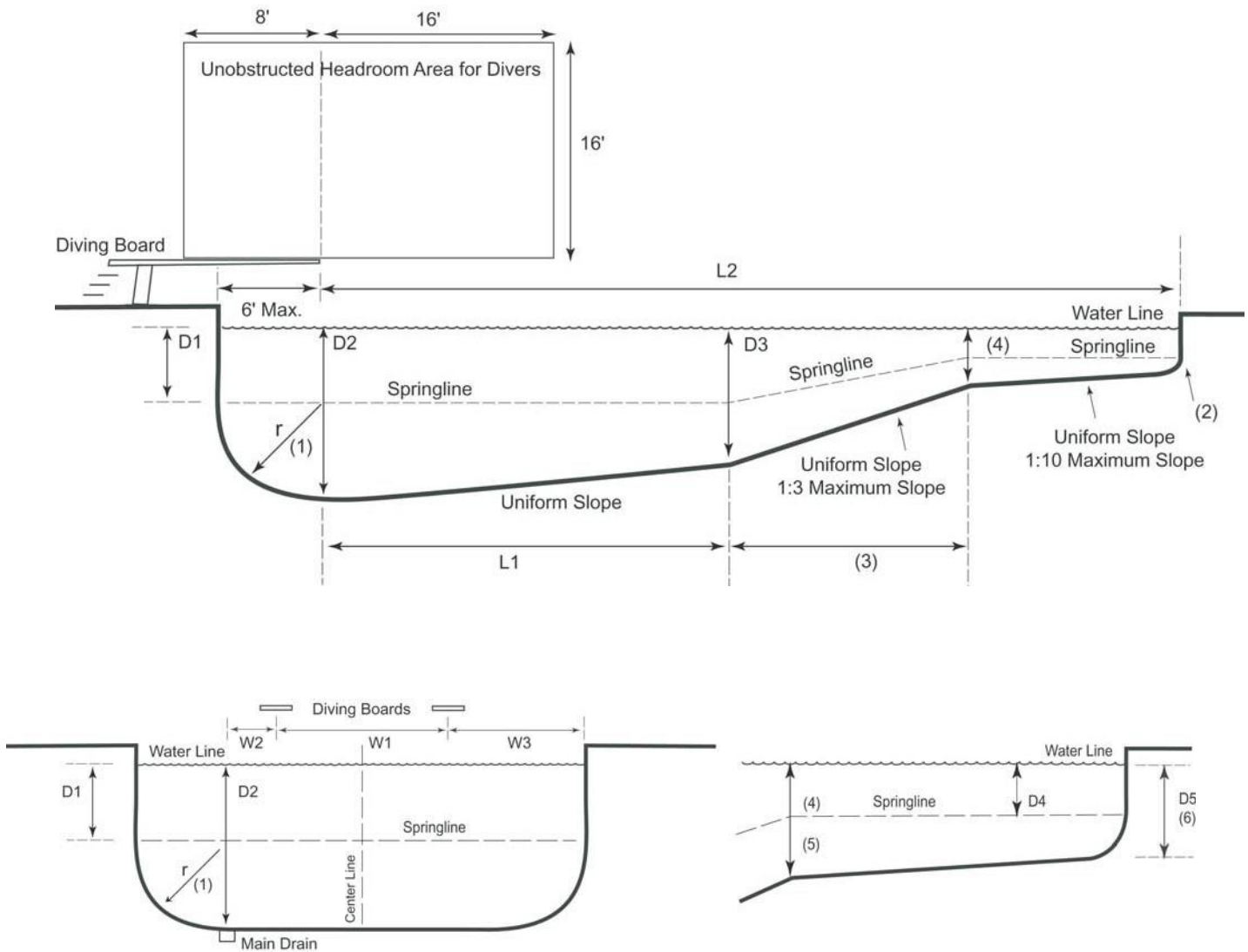
Transverse Section Deep End through Main Drain
